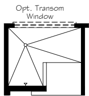
OPTIONAL L-SHAPED SHOWER LAYOUT WITH ZERO THRESHOLD
