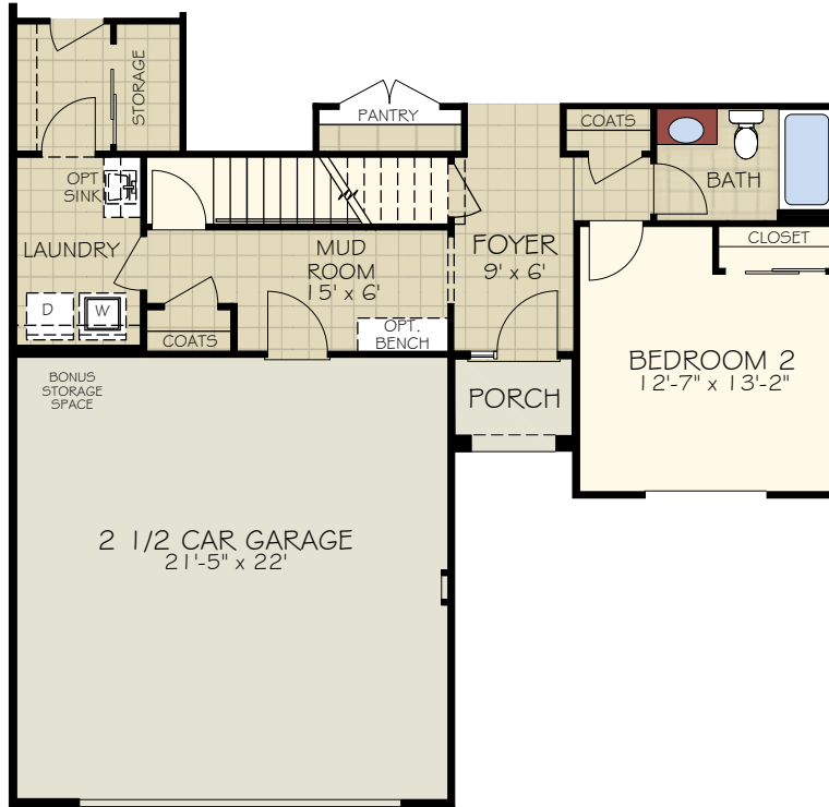
FIRST FLOOR PLAN W/ BONUS SUITE
