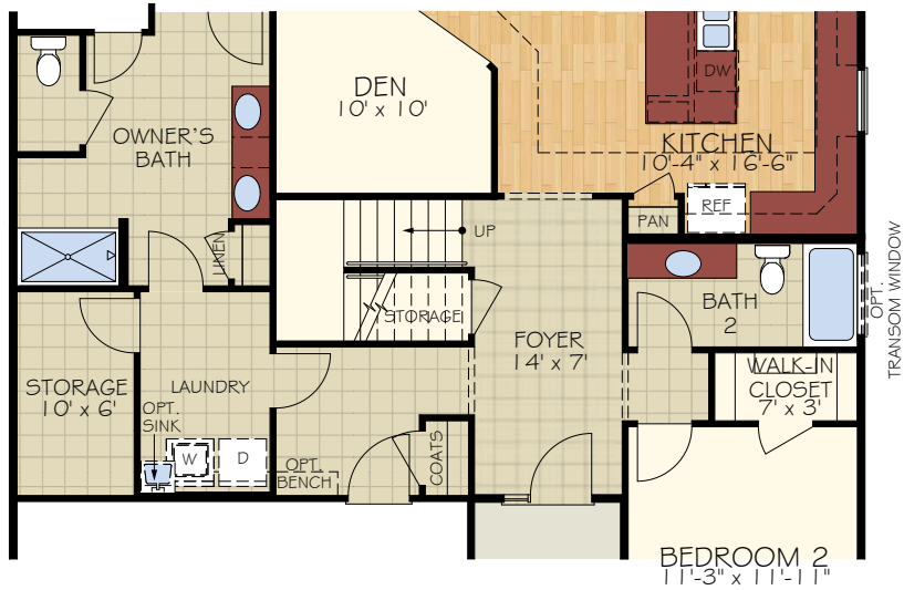
FIRST FLOOR PLAN W/ BONUS SUITE
