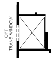
OPTIONAL UNIVERSAL SHOWER LAYOUT W/ ZERO THRESHOLD
