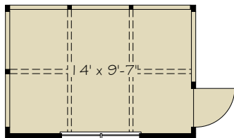
OPTIONAL OWNER SCREENED PORCH
