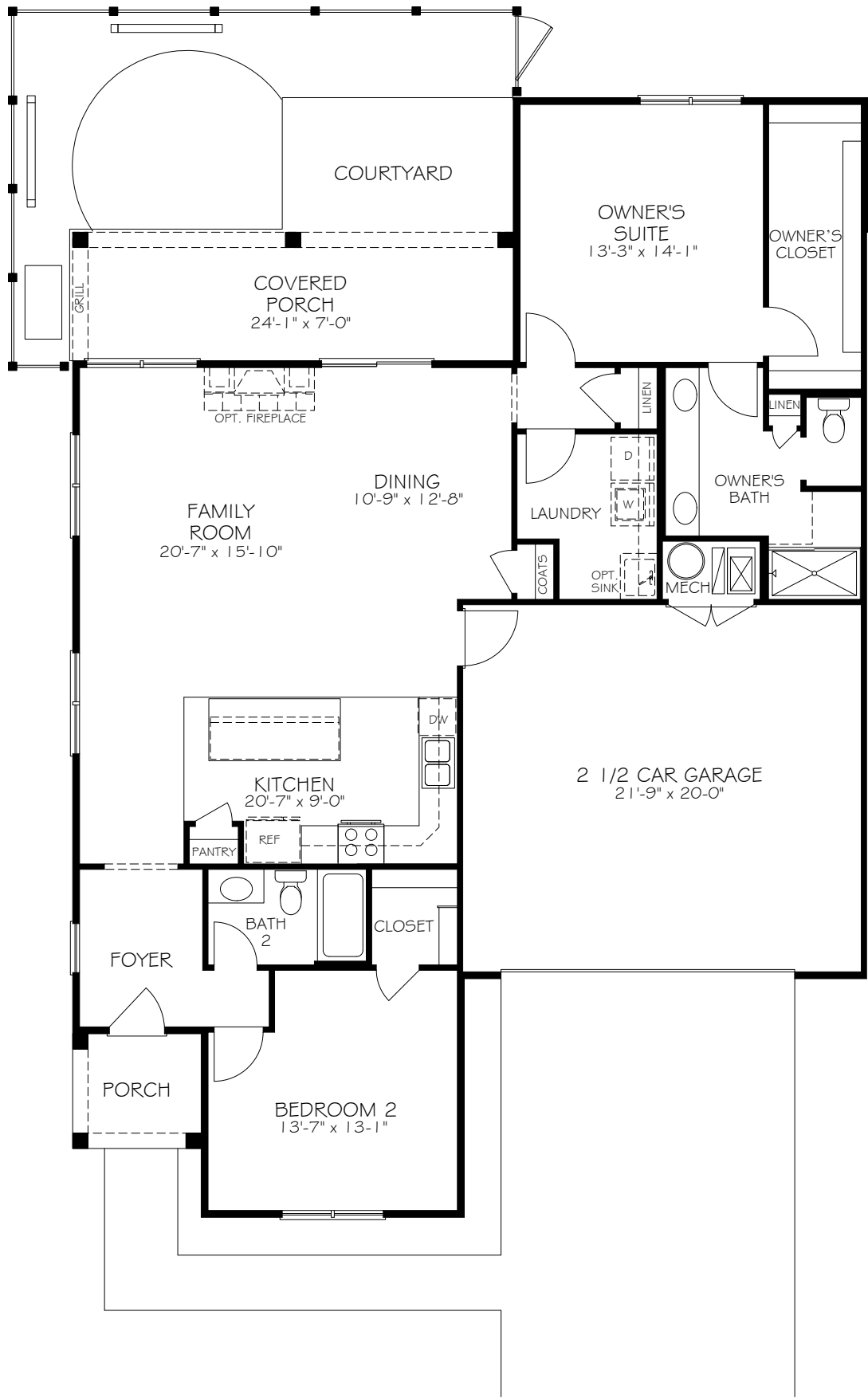
FIRST FLOOR
