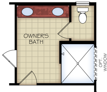
OPT. UNIVERSAL SHOWER LAYOUT WITH ZERO THRESHOLD
