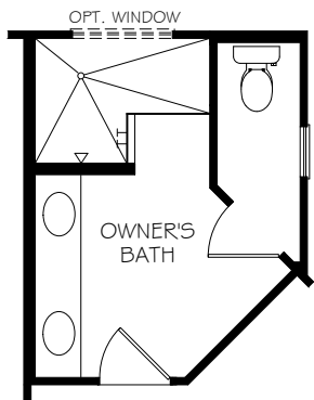
OPTIONAL L-SHAPED SHOWER LAYOUT WITH ZERO THRESHOLD
