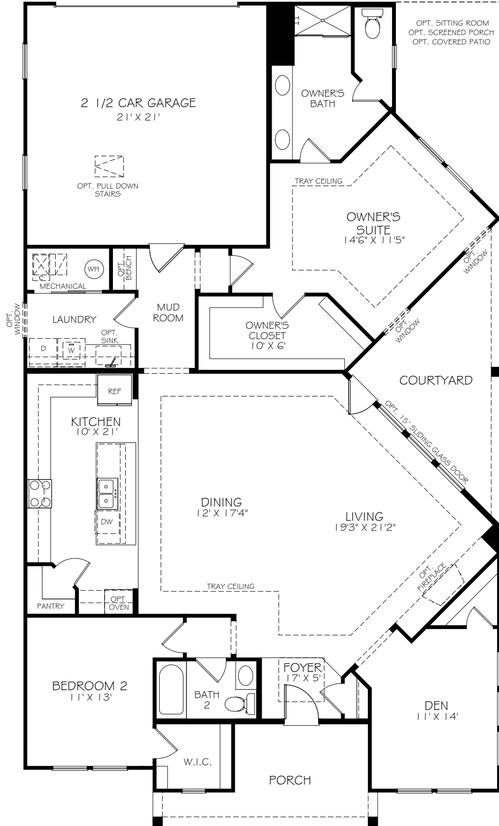
FIRST FLOOR
