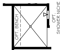
OPT. UNIVERSAL SHOWER LAYOUT WITH ZERO THRESHOLD
